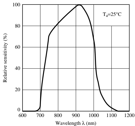
Fig.12 Spectral Sensitivity
